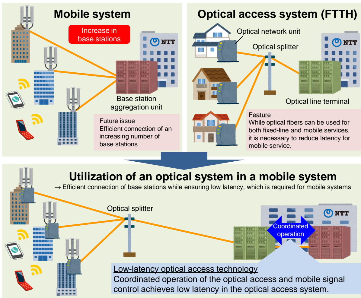
Fig. 1 Utilization of optical access systems in a mobile system
